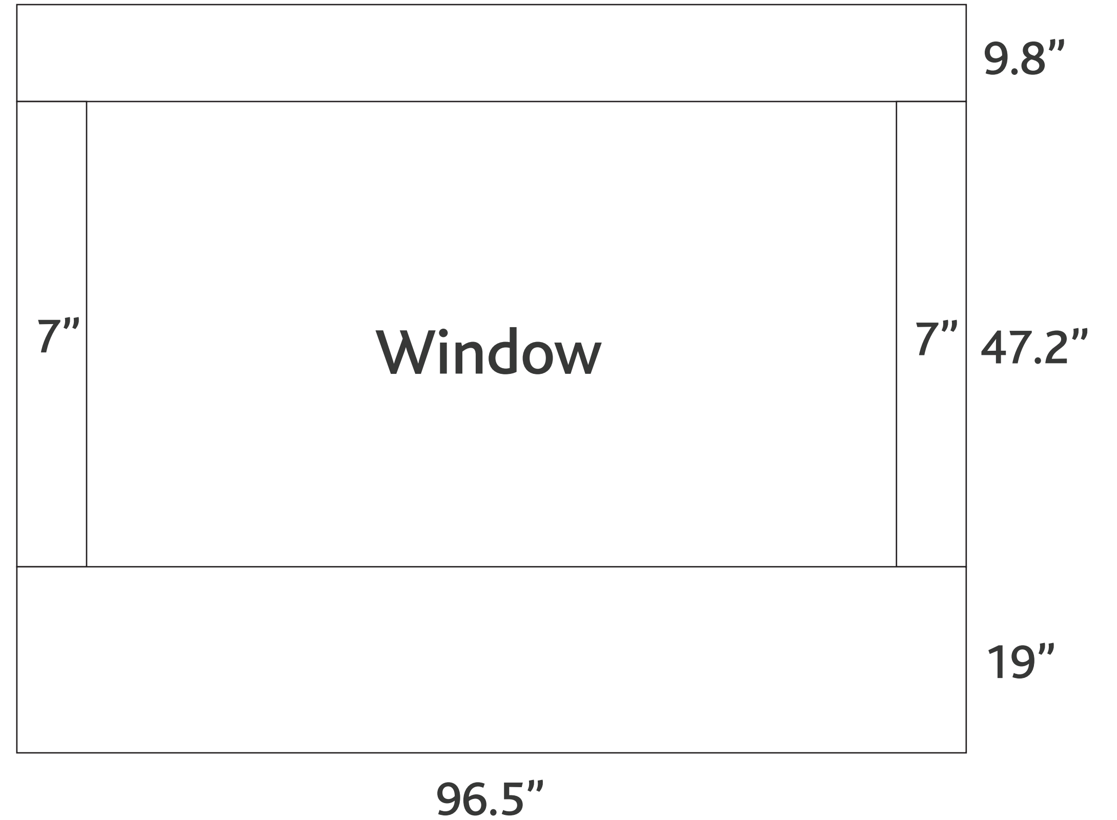
8ft Window Wall
